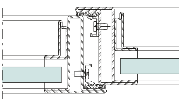
Face-fitted profile view
