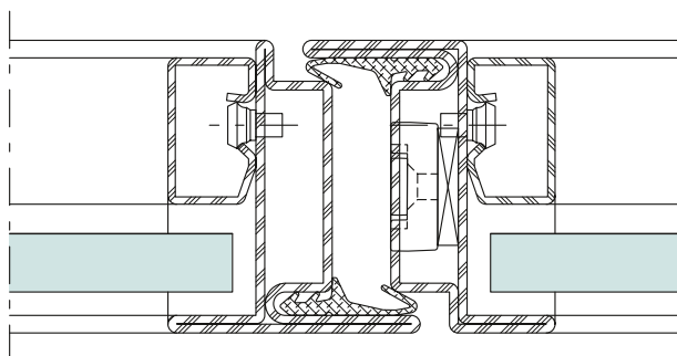
Flush-fitted profile view
