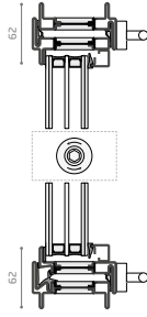
Vertical pivot window frame with constant sections around the perimeter and concealed hinges.
