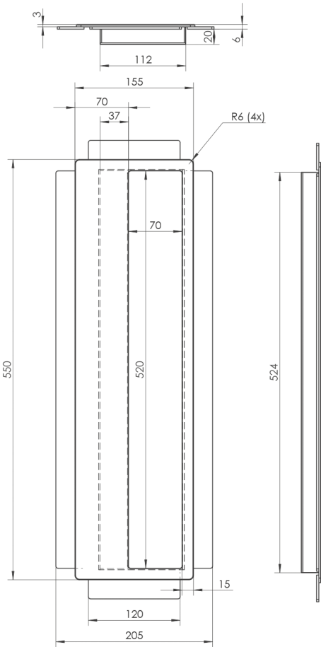
K1L - faced with the door panel
