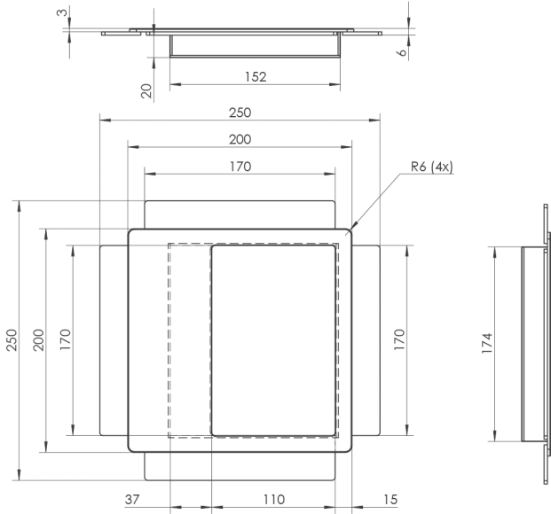
K1L - faced with the door panel
